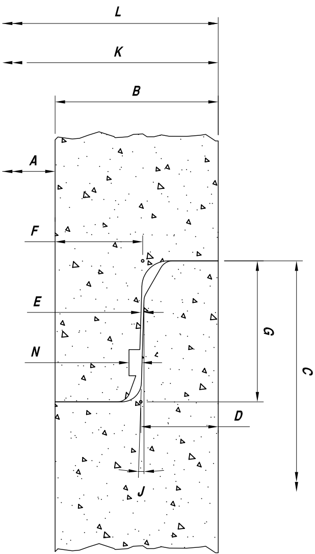
GROOVED JOINT DETAIL
