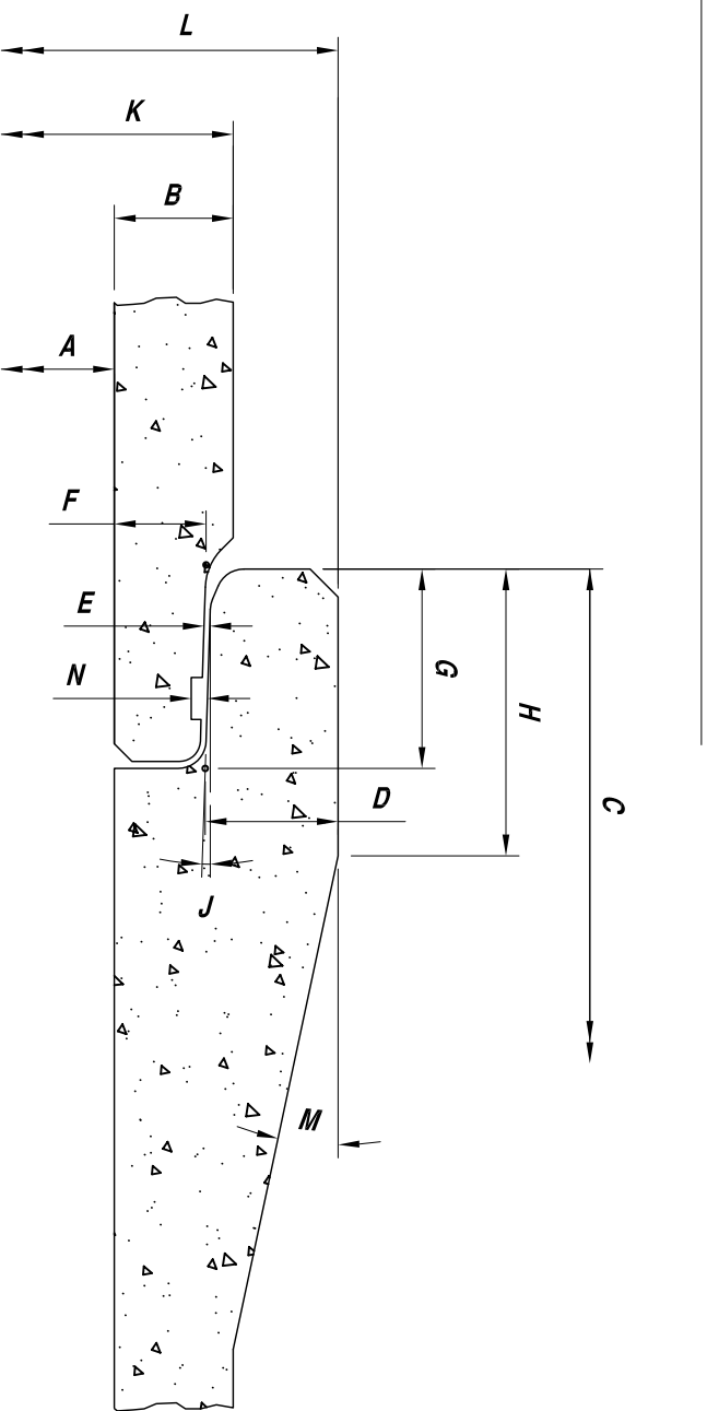
GROOVED JOINT DETAIL
